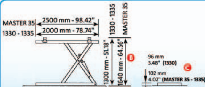
EH ELECTROHYDRAULIC
